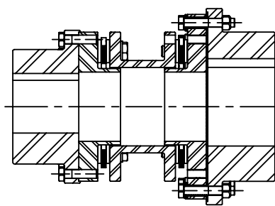
DIEI Type with Electrical Insulation
