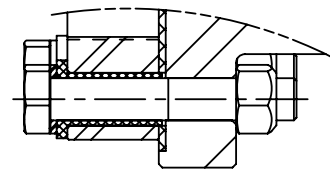
DIEI Type with Electrical Insulation
