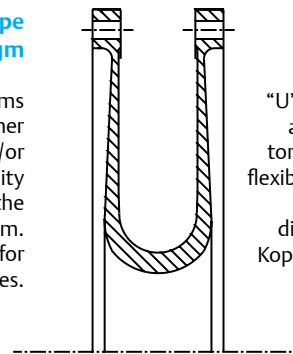
"U" Type Diaphragm
